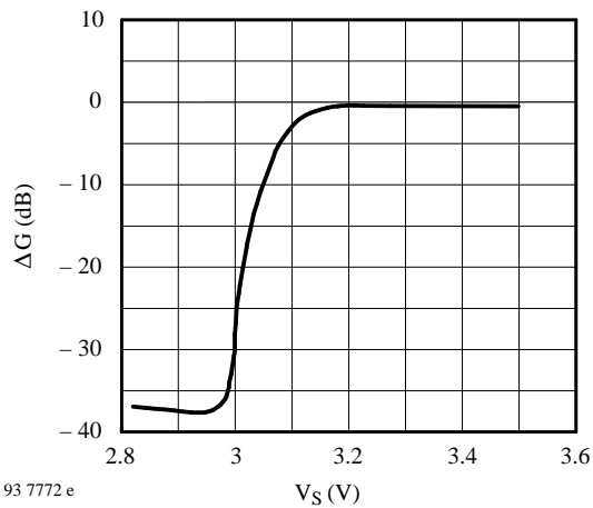
Figure 16. Receive attenuation gain versus V_S
