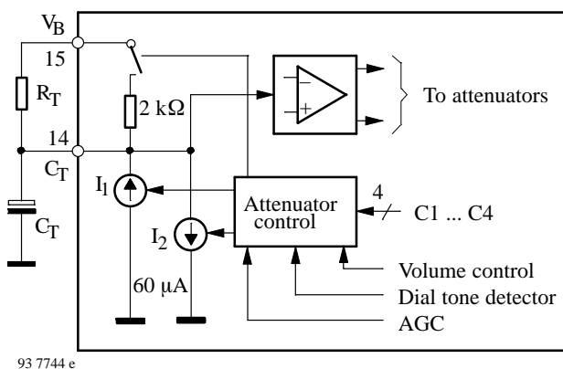
Figure 7. C T Attenuator control block circuit
